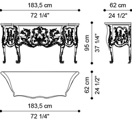
DRAWER UNIT J.WAL-21
