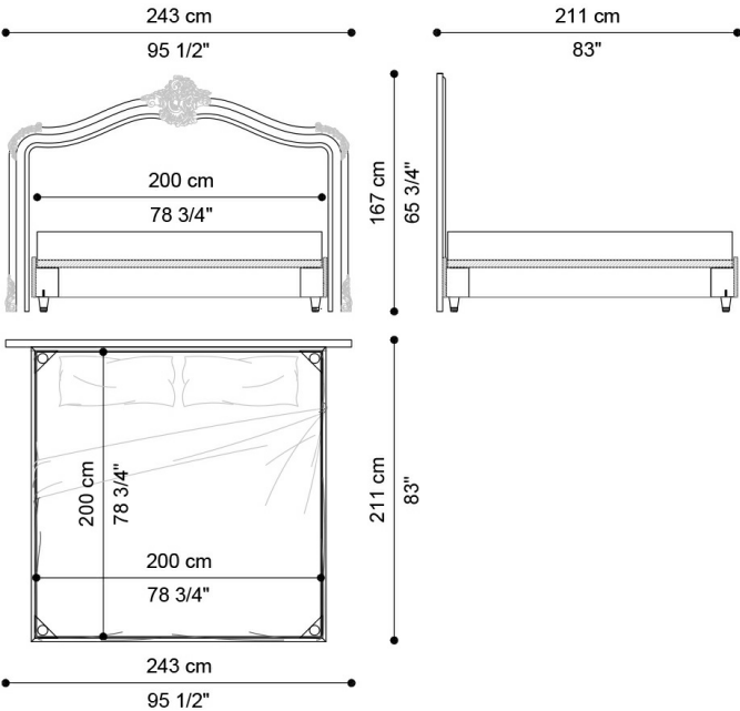
BED - FOR MATTRESS 200 X 200 CM J.CHN-02B
