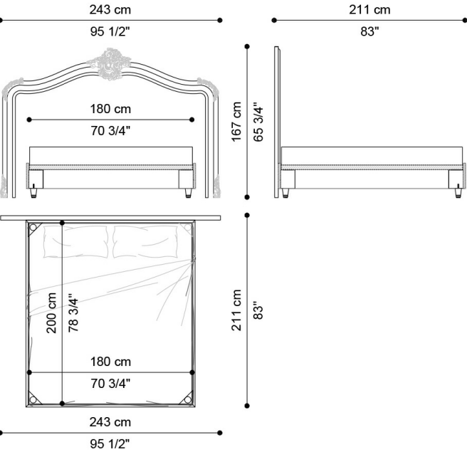
BED - FOR MATTRESS 180 X 200 CM J.CHN-02
